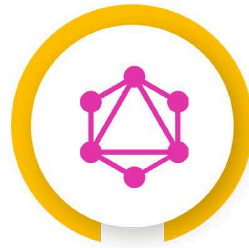
GRAPHQL
