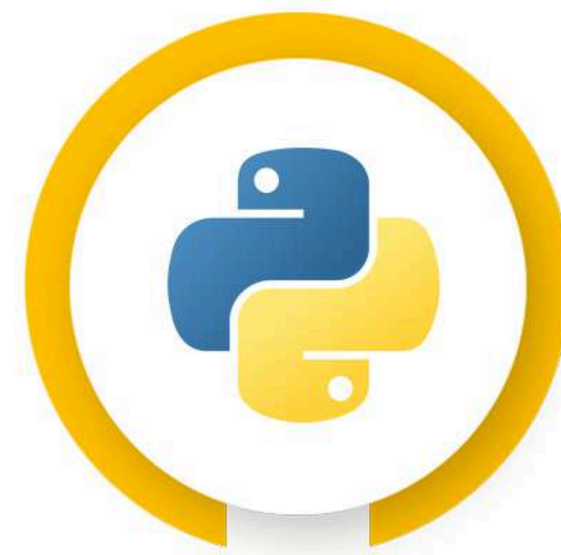
PYTHON
