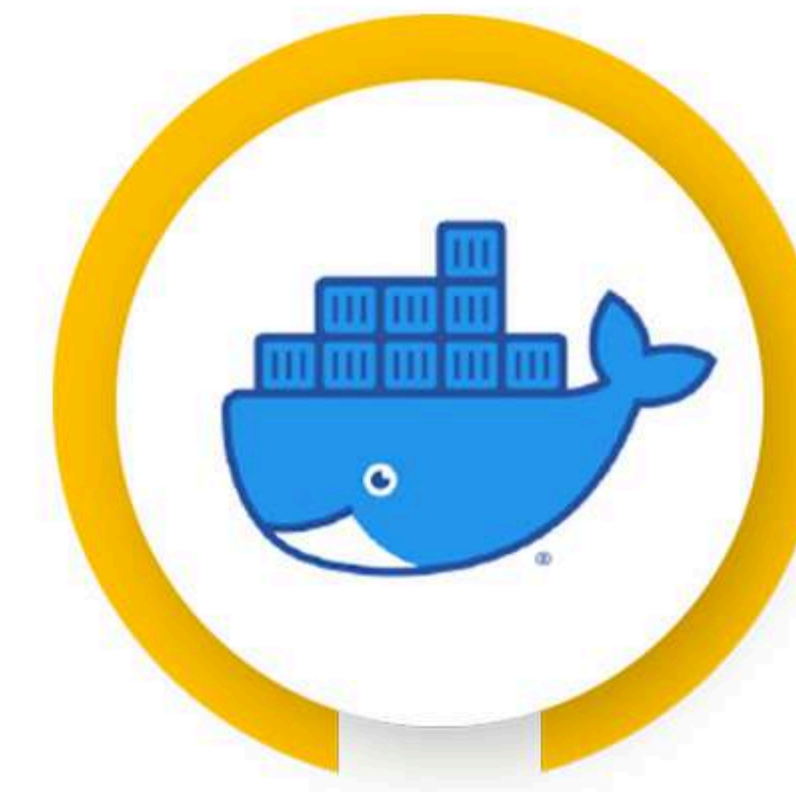
DOCKER
