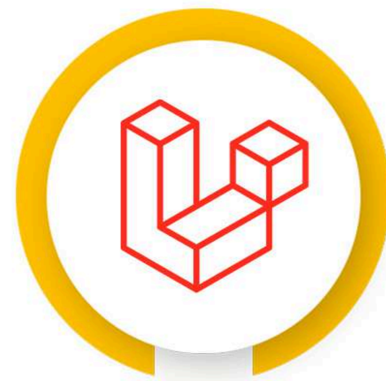
LARAVEL
