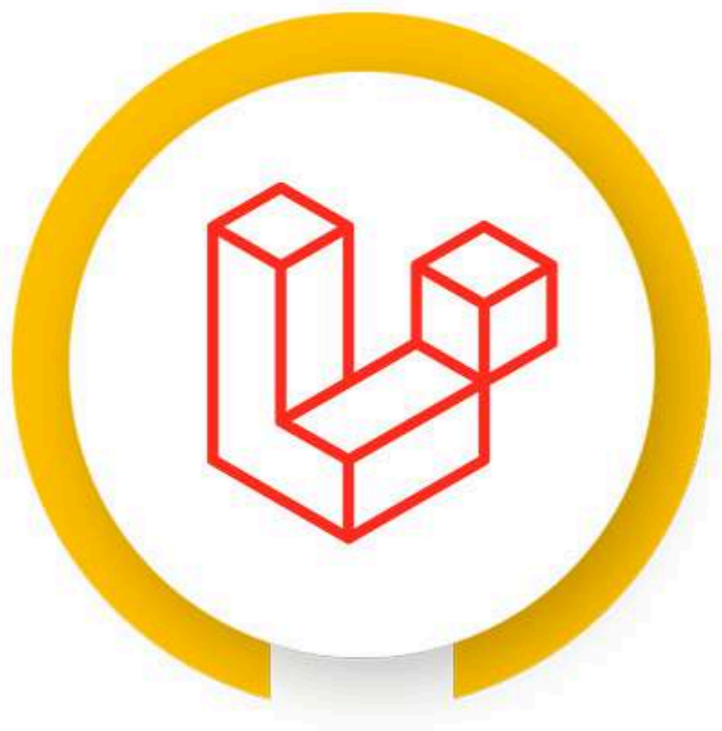
LARAVEL
