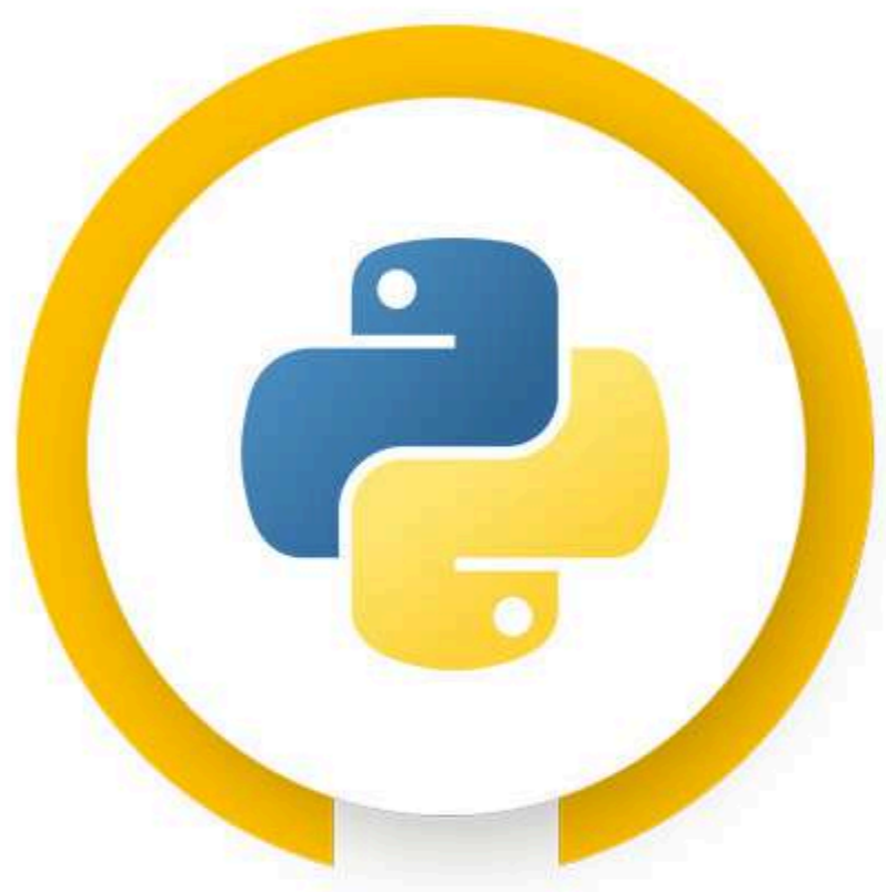
PYTHON
