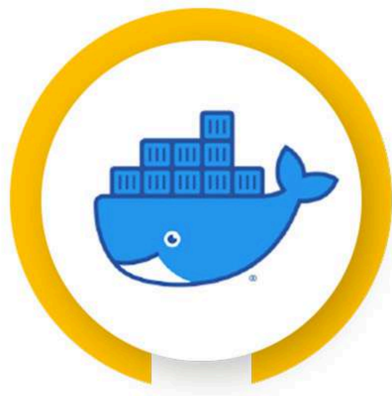
DOCKER
