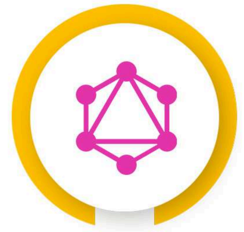
GRAPHQL
