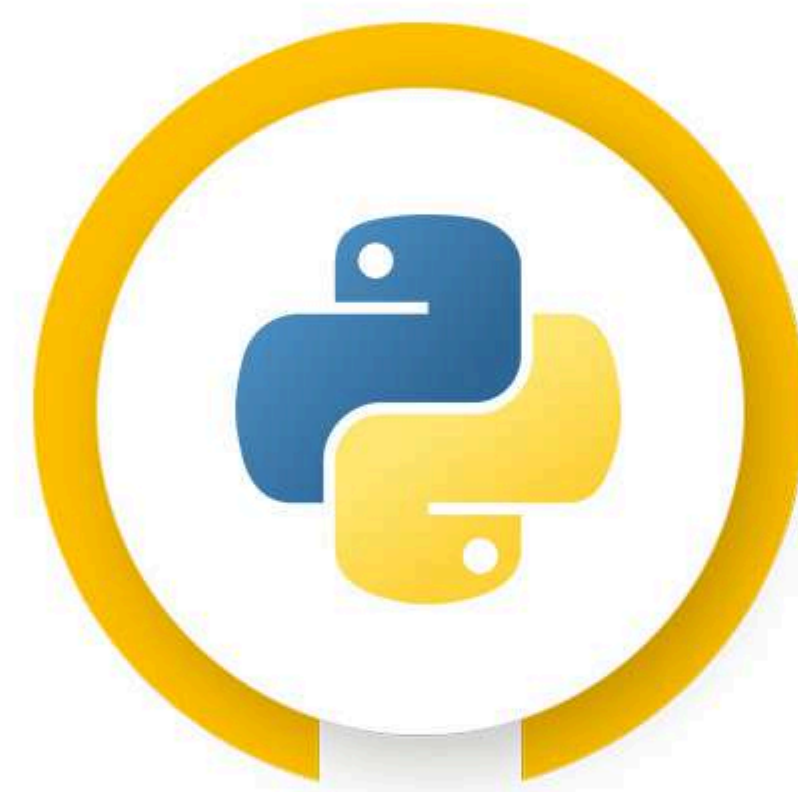
PYTHON
