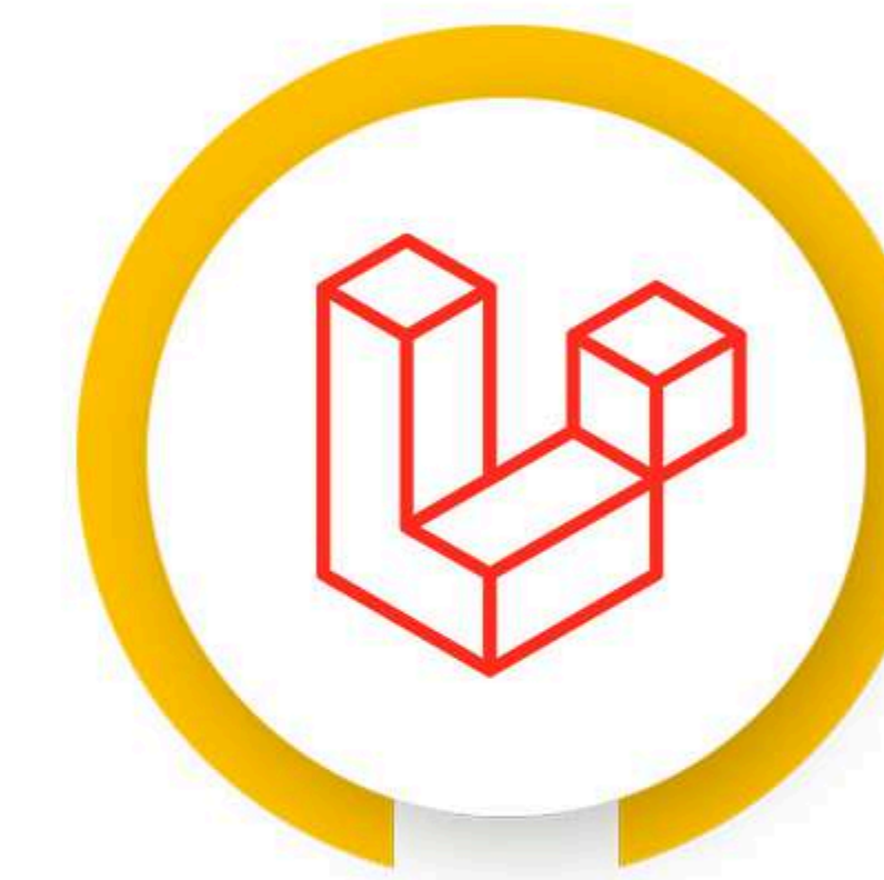
LARAVEL
