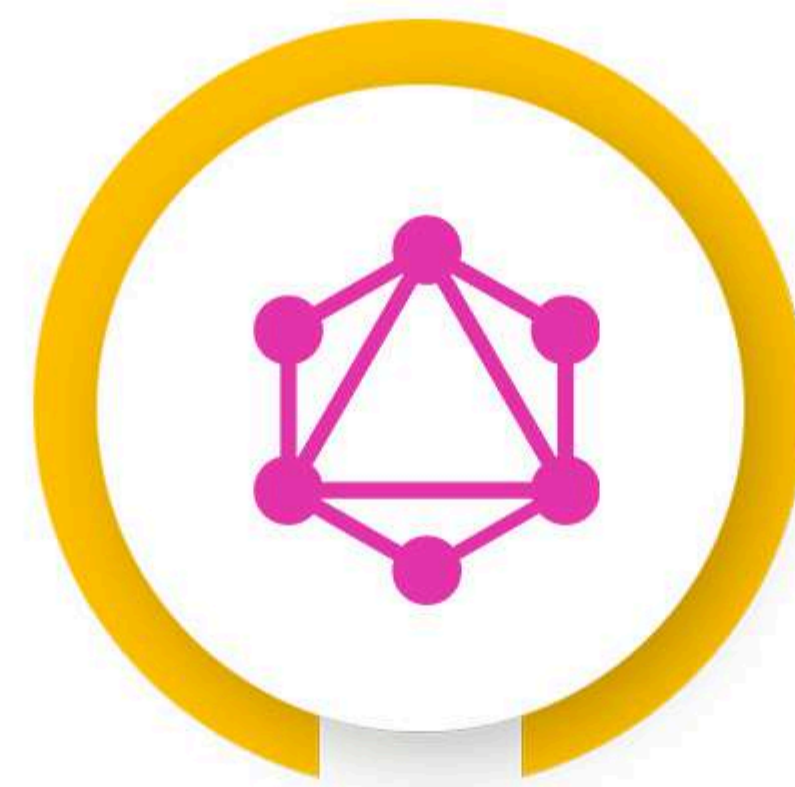
GRAPHQL
