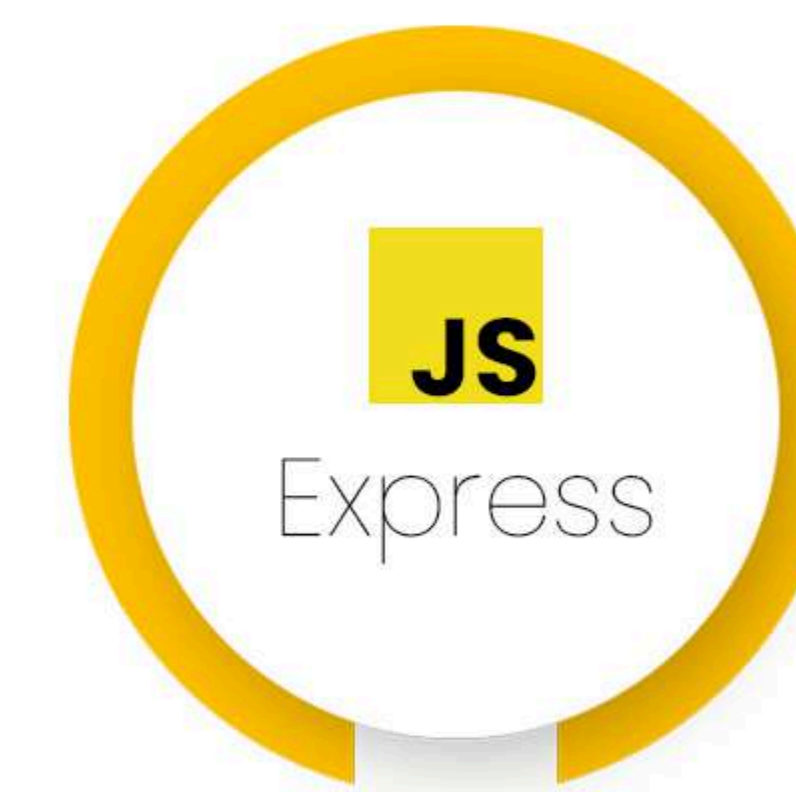
EXPRESS.JS
