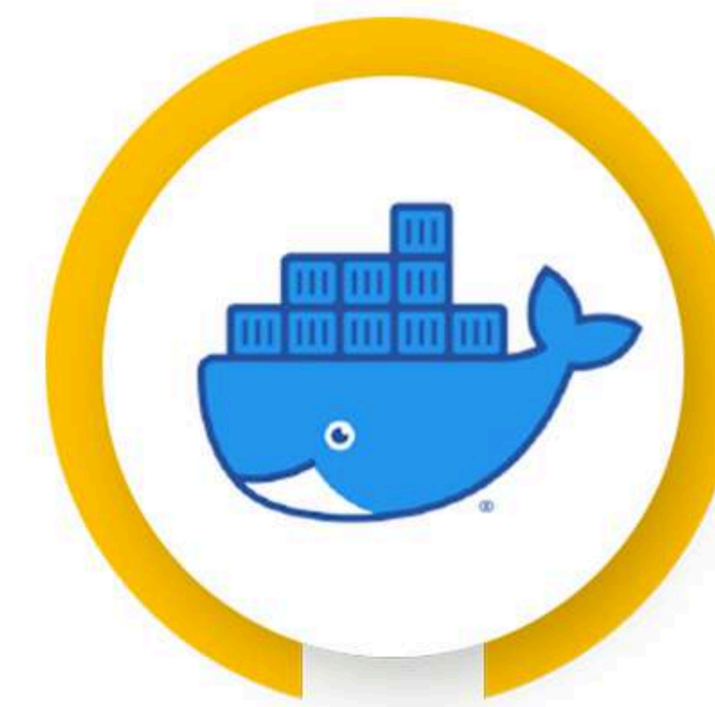
DOCKER
